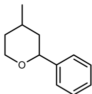
Tetrahydro-4-methyl-2-phenyl-2H-pyran
